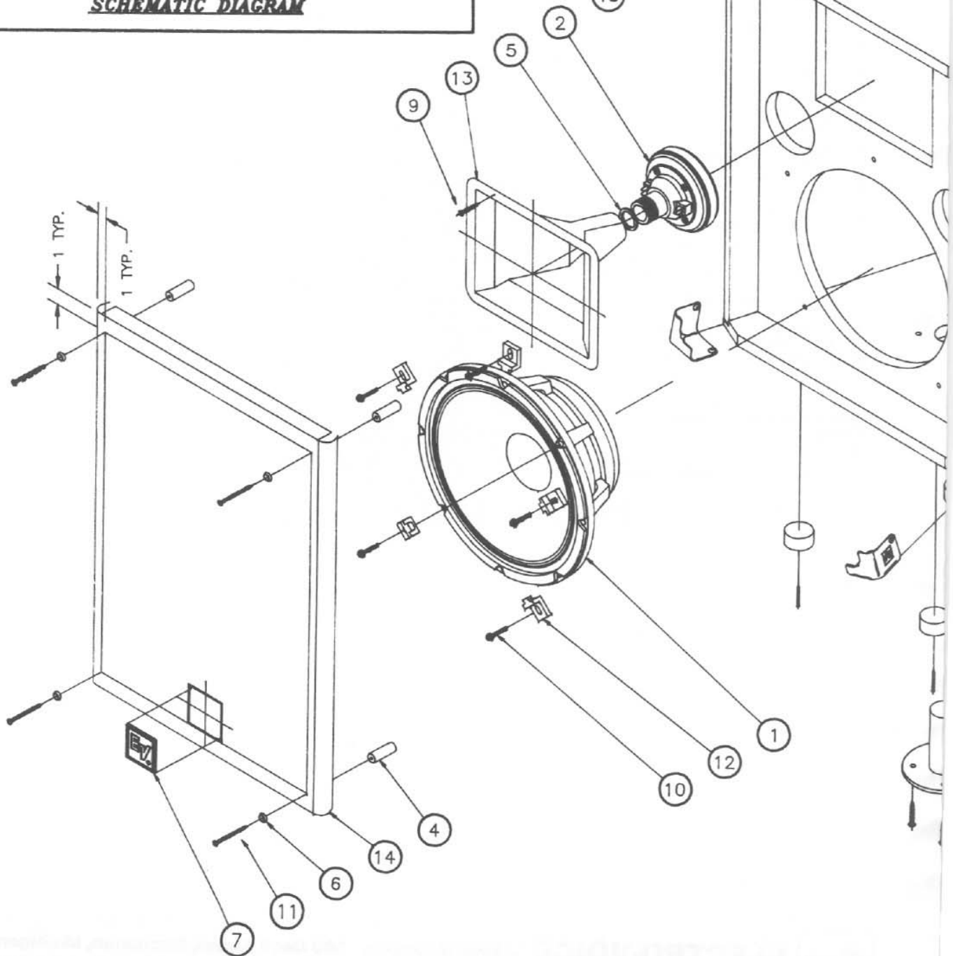
SCHEMATIC DIAGRAM
