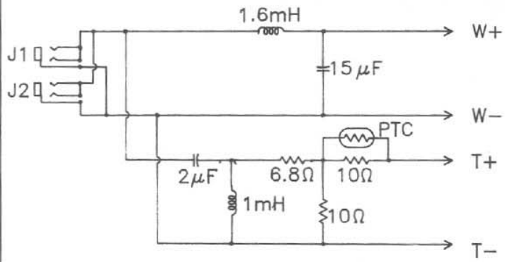
SCHEMATIC DIAGRAM
